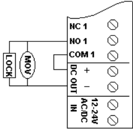
CCTV/DOORBELL and Fail Secure Lock Controlled by KE-265
