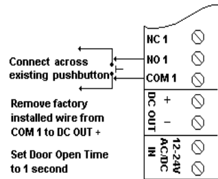
Garage Door/Gate Drive Controlled by KE-265
