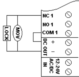
Fail Safe Lock Controlled by KE-265
