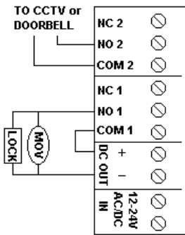
Fail Safe or Fail Secure Lock Controlled by KE-265 And Powered by External Power Supply
